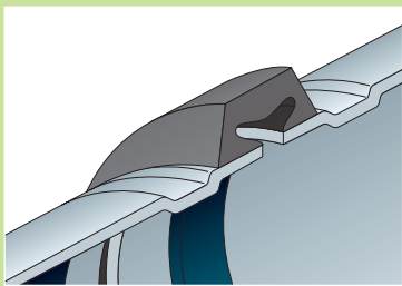
First seal C-shape rubber gasket naturally seals on pipe ends.
