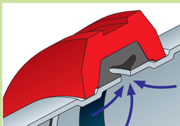
Third seal The system pressure or vacuum will then maximize the leak-tight seal.
