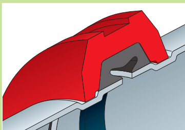
Second seal The housings compress the gasket to increase the sealing capacity.
